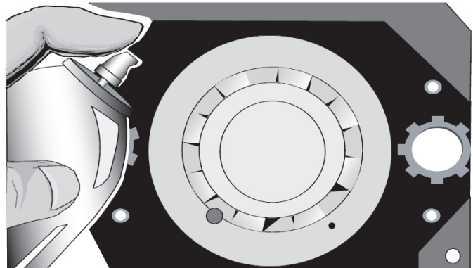
Above: For factory recommended functional testing, spray the proper test gas directly at the detector head from a distance of 12 inches for 2 seconds.
